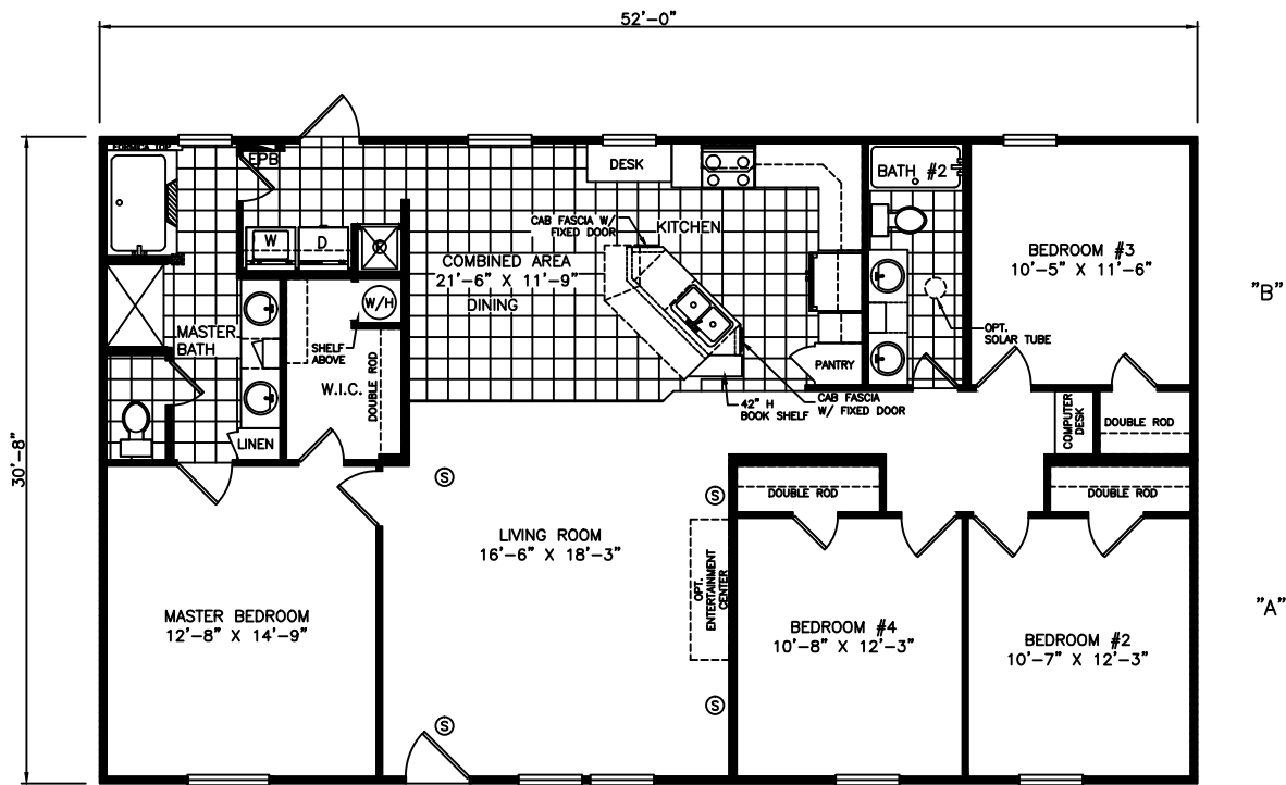
MODEL B-325642B BOX SIZE=30'-8" x 52'-0" 4 BEDROOMS / 2 BATH (1602 SQ. FT.)
